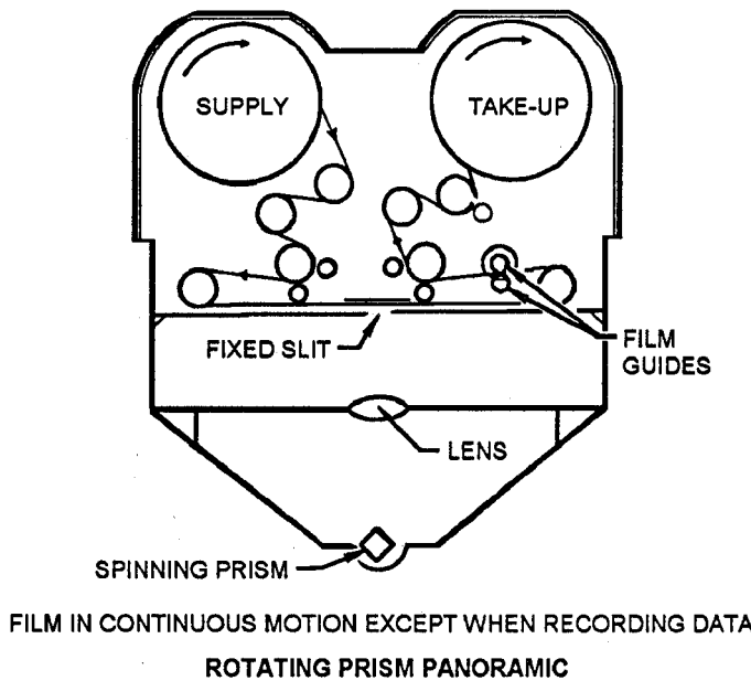
Figure 6-18.—Special format panoramic cameras.
